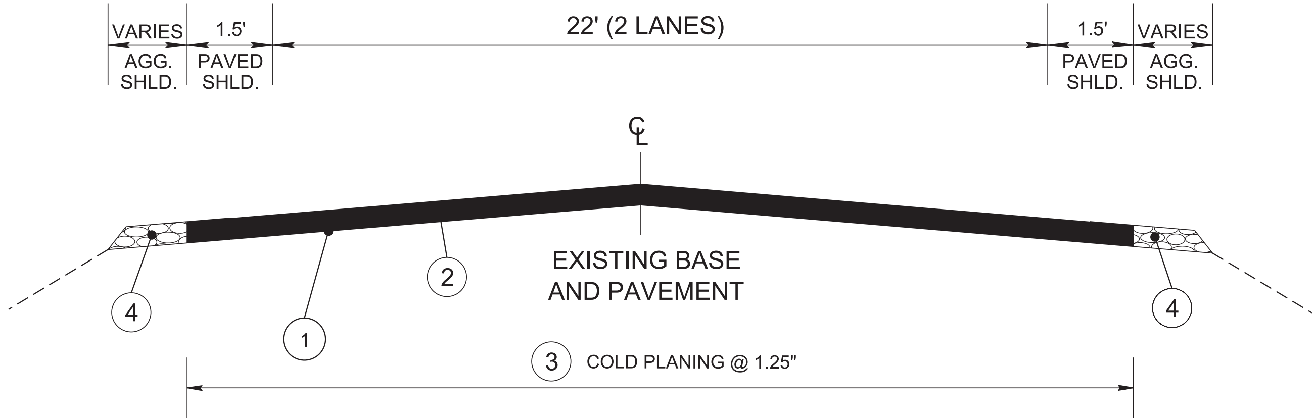
CHEATHAM COUNTY SR-49 TYPICAL SECTION
